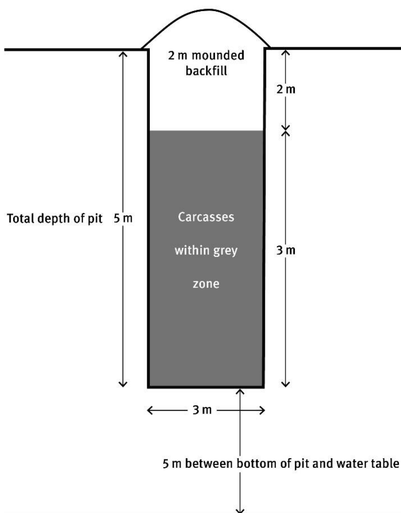
Figure 1 – Traditional trench style burial pit
