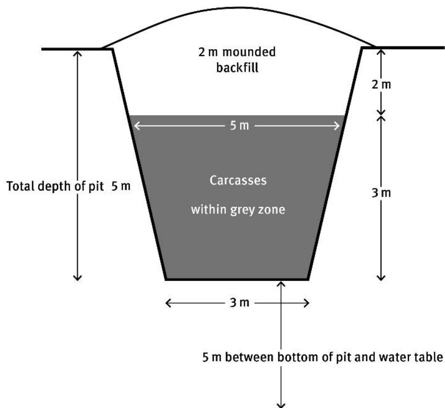
Figure 2 – Traditional battered burial pit
